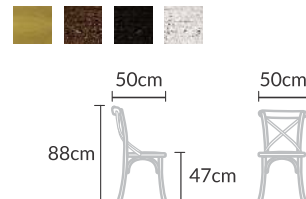
Cadeira Paris Ref. 5392 - OAK Ref. 5534 - Canela Ref. 5615 - Preto Provençal Ref. 5456 - Branco Provençal
